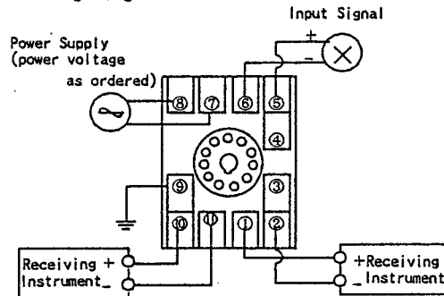
Fig.6 Wiring Diagram
