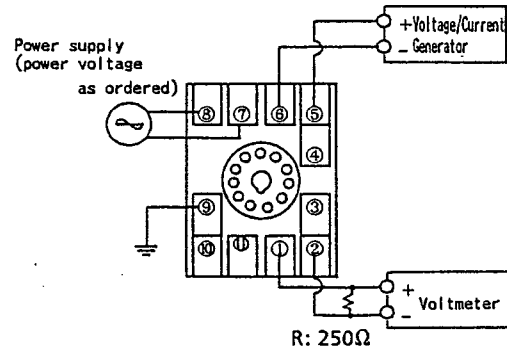
Fig.7 Wiring of Calibration Equipment
