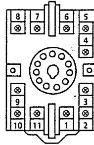
Fig.6 Wiring Diagram
